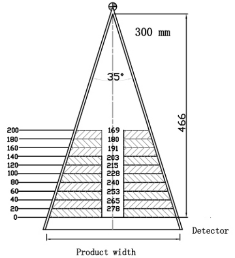
X12 Beam Size Diagram
